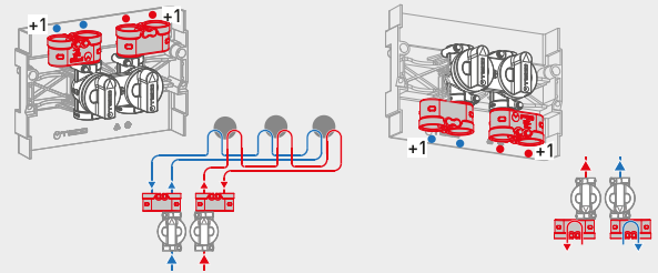
TWIN 1 FITTING COD. KA00F10001
